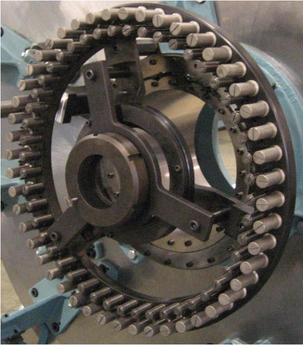
Flex Mandrel Preform Tooling
