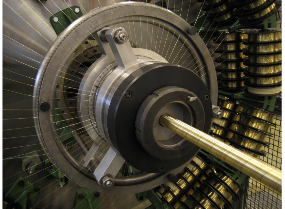
Preform Tooling for Large Diameter Hose
